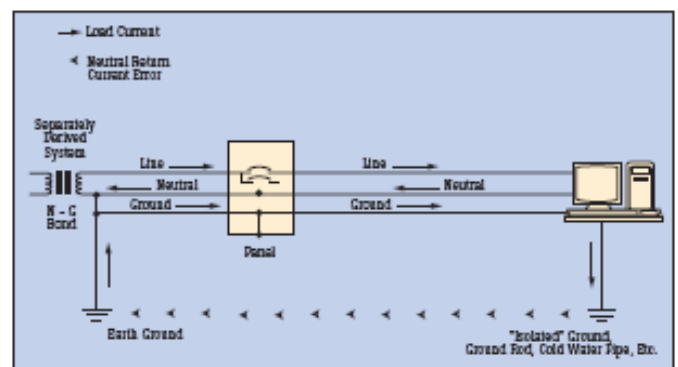
Figure 2 Isolated ground rod can cause ground loops. Common problem with CNC machine tool installations
