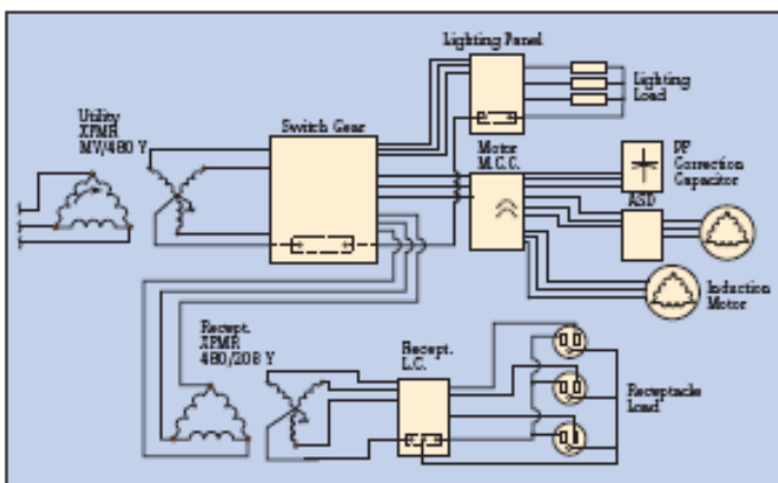
Figure 1 Simplified electrical distribution system typical of commercial and industrial facilities
